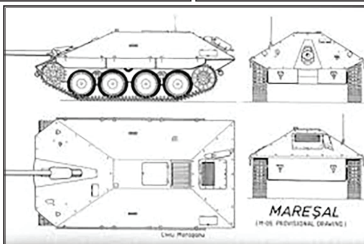
Vânătorul de tancuri „Mareșal” (sursa: https://gmic.co.uk/topic/72329-actual-sketching-of-a-mare%C8%99al-tank-destroyer/ )
